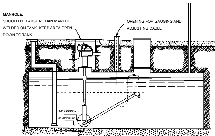
Figure 1.2 Floating suction installation
