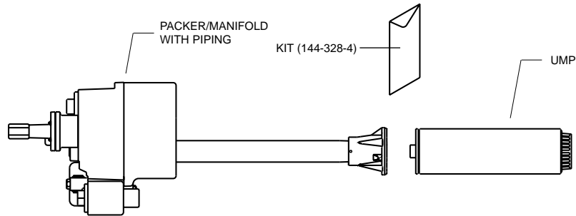
Figure 2.1 Attaching the UMP
